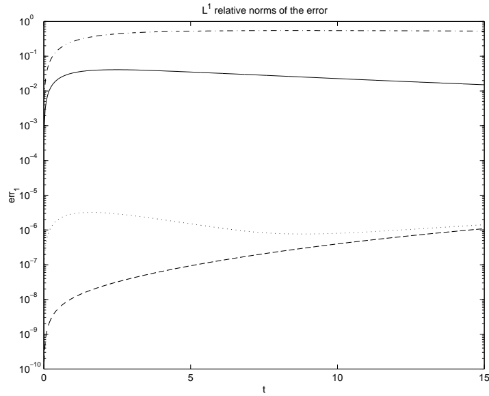
Figure 1: Relative L^1 norm of the error for Test # 1. V_{\max} = 6.6 . Number of modes: 8^2 (dot-dash), 16^2 (continuous line), 32^2 (dotted line), 64^2 (dashed line).
