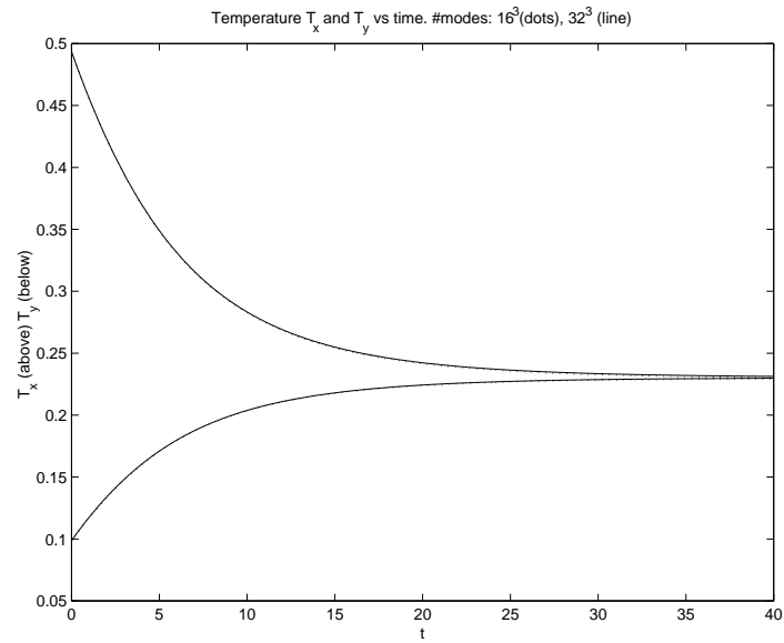
Figure 4: Temperature evolution for Test # 2. Number of modes: 16^3 (dotted line) and 32^3 (continuous line).
