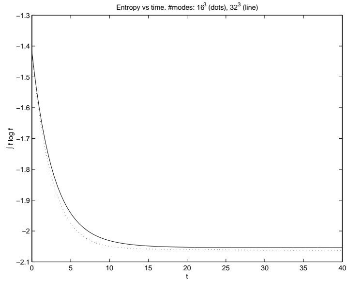
Figure 3: Entropy decay for Test # 2. Number of modes: 16^3 (dotted line) and 32^3 (continuous line).
