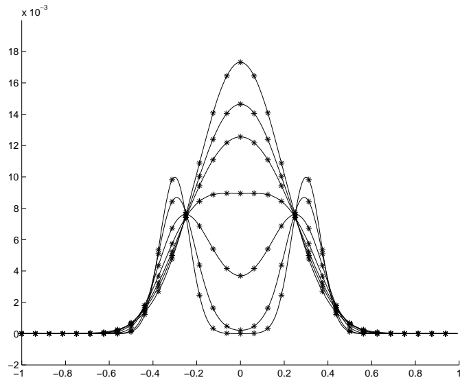
Figure 6: Cross section of the distribution function at different times, for Test # 3. Number of modes: 32^3 . Grid values (*), trigonometric reconstruction (continuous line).
