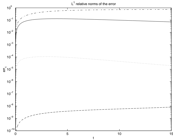
Figure 2: Relative L^1 norm of the error for Test # 1. V_{\max} = 7.7 . Number of modes: 8^2 (dot-dash), 16^2 (continuous line), 32^2 (dotted line), 64^2 (dashed line).
