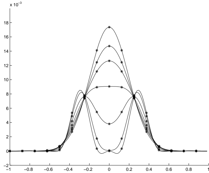
Figure 5: Cross section of the distribution function at different times, for Test # 3. Number of modes: 16^3 . Grid values (*), trigonometric reconstruction (continuous line).
