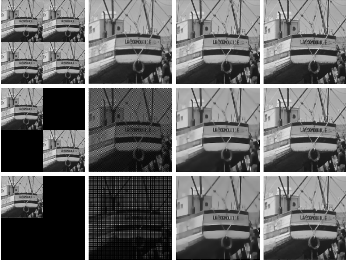
FIGURE 2. Super-resolution image reconstruction using 2 \times 2 sensors for the “boat” image. Columns (from left to right) are the available low-resolution images, the observed high-resolution images, the reconstructed high-resolution images by the analysis-based approach (3.3), and the reconstructed high-resolution images by the balanced approach (1.5). The PSNR values of the reconstructed images in the third column (analysis-based approach) are 31.7281, 28.0557 and 22.4243 respectively, and those in the fourth column (balanced approach) are 29.2638, 29.1752 and 24.5309 respectively.
