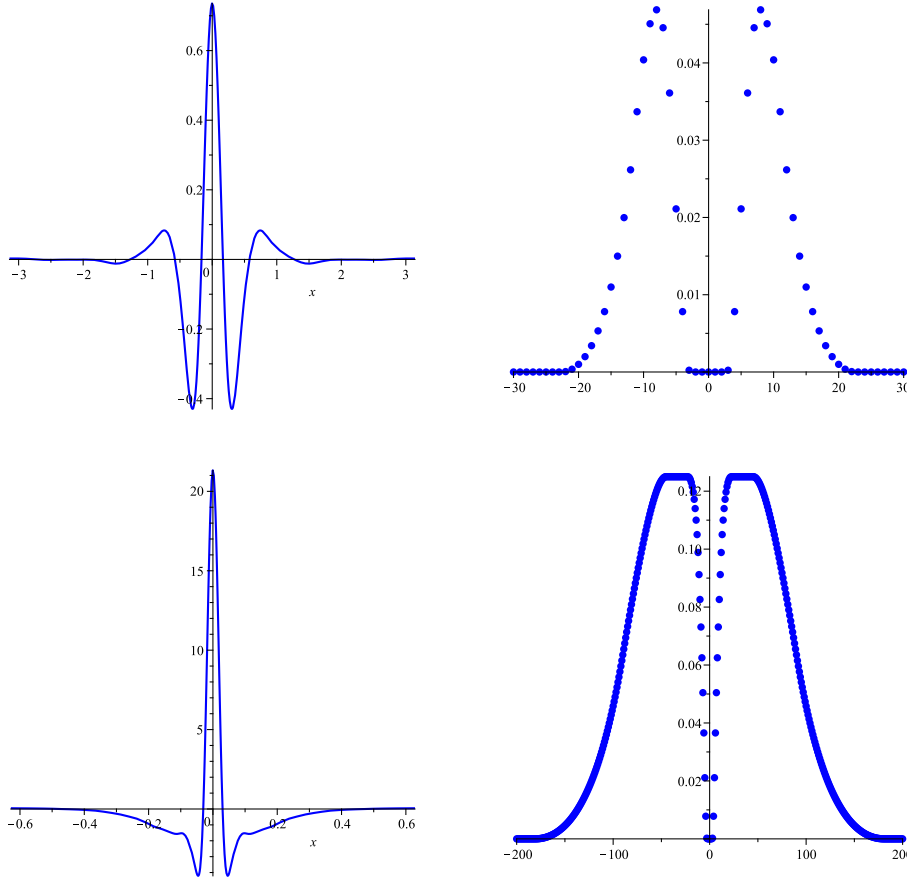
FIGURE 1. Plots of \psi_k (top left) and \widehat{\psi}_k (top right) defined by (3.11) and (2.8) for D = 2 , k_0 = 5 and k = 8 , and the corresponding \widetilde{\psi}_k (bottom left) and \widehat{\widetilde{\psi}}_k (bottom right) from (3.5) as in Example 3.2.
