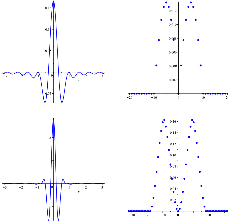
FIGURE 2. Plots of \psi_k (top left) and \widehat{\psi}_k (top right) defined by (3.14) and (2.11) for L_k = k^2 , N = 5 , k_0 = 7 and k = 12 , and the corresponding \widetilde{\psi}_k (bottom left) and \widetilde{\widehat{\psi}}_k (bottom right) from (3.1) as in Example 3.4.
