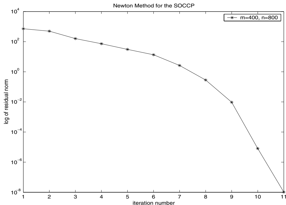
Figure 1. The logarithm of residual norm \|H(z)\| by iterations.
