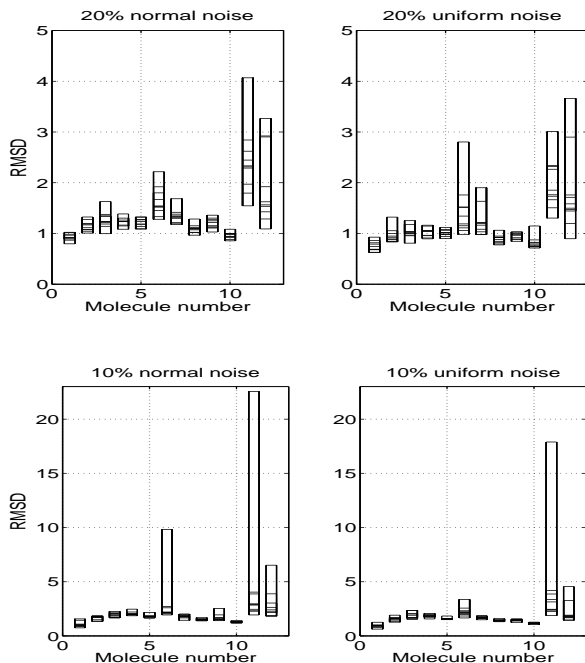
FIG. 5.1. For each molecule, ten random inputs were generated with different initial random number seeds. We plot the the RMSDs of the ten structures produced by DISCO against the molecule number. (top left) 30% short-range distances, 20% normal noise (top right) 30% short-range distances, 20% uniform noise (bottom left) 20% short-range distances, 10% normal noise (bottom right) 20% short-range distances, 10% uniform noise.
