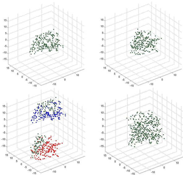
FIG. 4.1. Since the number of atoms is too large ( n = 402 > \text{basis size} = 300 ), we divide the atoms into two subgroups; see Fig. 3. We solve the subgroups independently (top left and right). The subgroups have overlapping atoms, which are colored in green (bottom left). The overlapping atoms allow us to align the two subgroups to form a realization of the molecule.
