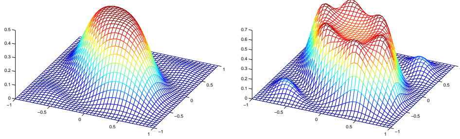
Figure 1. Primary and dual Gabor windows of Example 4.10.
