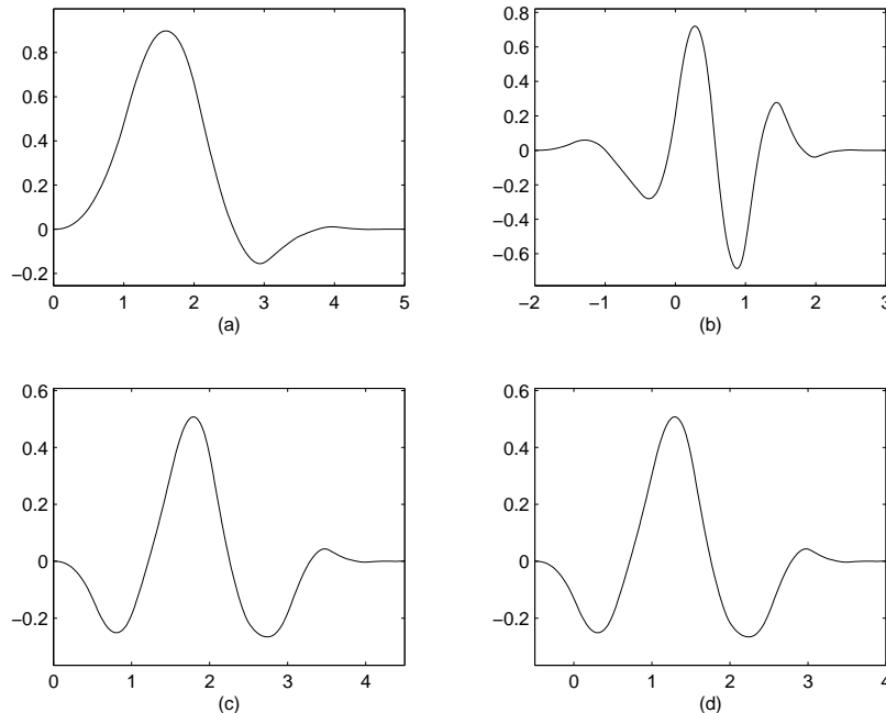
Figure 5. (b), (c) and (d) are the graphs of the mother wavelets in Example 2.20 of the Type I pseudo-spline tight framelets derived from the scaling function, pseudo-spline (4, 1), shown in (a). (See §3.1 for details)
