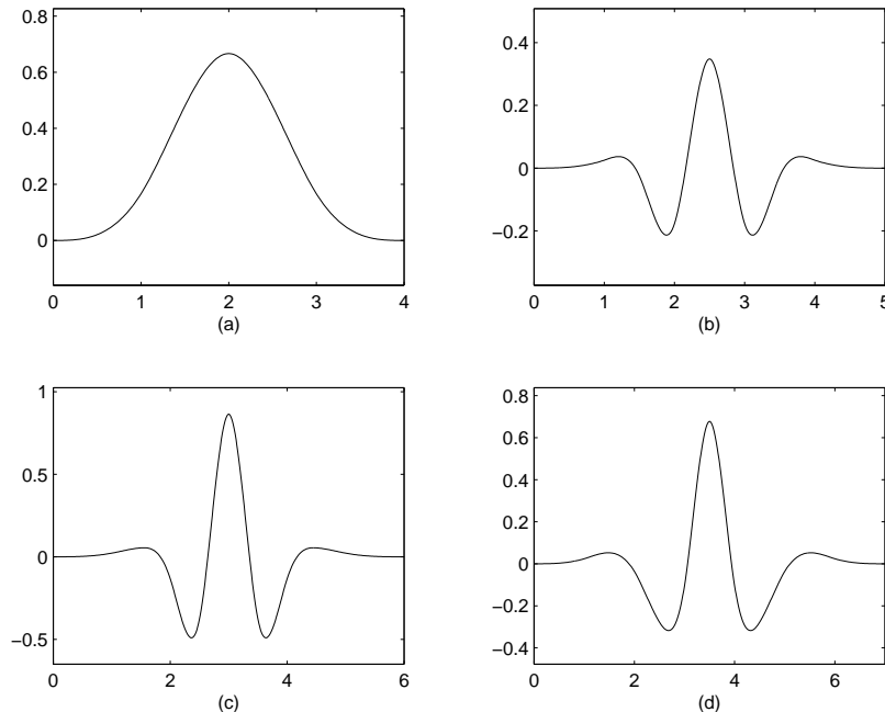
Figure 4. (b), (c) and (d) are the graphs of the symmetric mother wavelets derived from the cubic B-spline function (a) in Example 2.19. All the mother wavelets have 4 vanishing moments, hence the approximation order of the system is \min\{4, 8\} = 4 .
