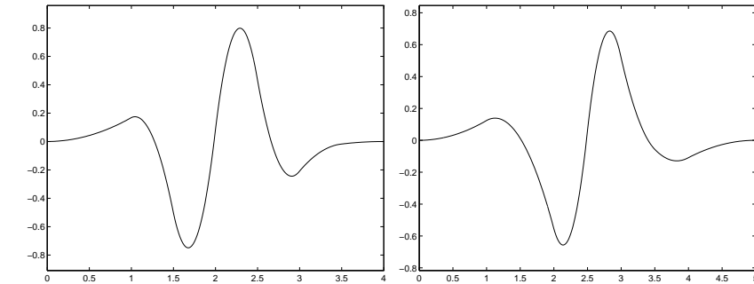
Figure 9. The graphs of the mother wavelets corresponding to (A.2) in Example A.1. The system provides approximation order 3 and has 3 vanishing moments. The filters are of lengths 6 and 8.
