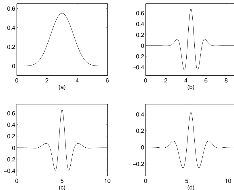
Figure 13. (b), (c) and (d) are the graphs of the symmetric mother framelets derived from the B-spline function of order 6 in (a) in Example A.4. The tight framelets has 6 vanishing moments, hence approximation order 6, as well.
