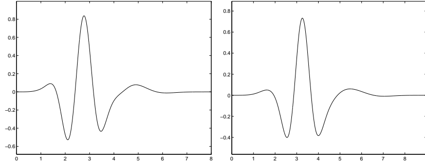
Figure 12. The graphs of the two (non-symmetric) mother wavelets in Example A.3. The tight framelet has approximation order 5 as well as vanishing moments of order 5. Note that the filters are 12- and 14-tap.
