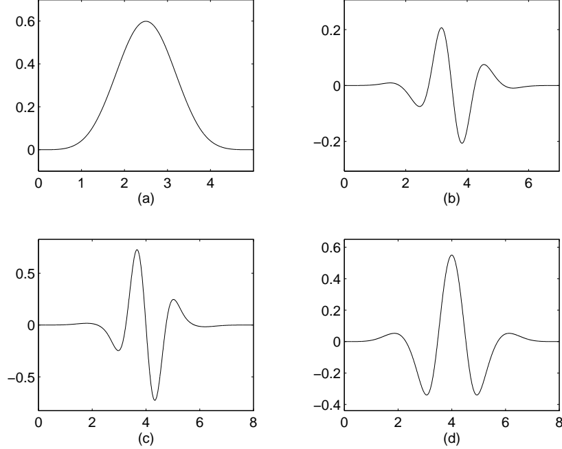
Figure 11. (b), (c) and (d) are the graphs of the symmetric mother wavelets derived from the B-spline function of order 5 in (a) in Example A.3. This tight framelet has vanishing moments of order 4, hence the approximation order is maximal, i.e., 5.
