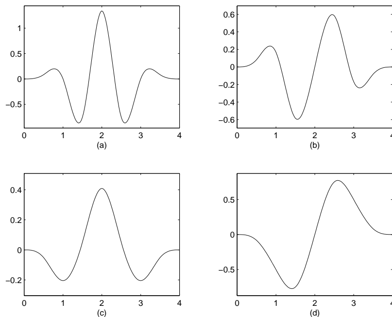
Figure 2. The graphs of the wavelet functions \psi_1, \psi_2, \psi_3, \psi_4 derived from the B-spline function of order 4 in Example 2.17; together, the four wavelets generate a tight framelet. Wavelet (d) has only one vanishing moment, hence the approximation order is 2, which is suboptimal since the corresponding MRA provides approximation order 4.
