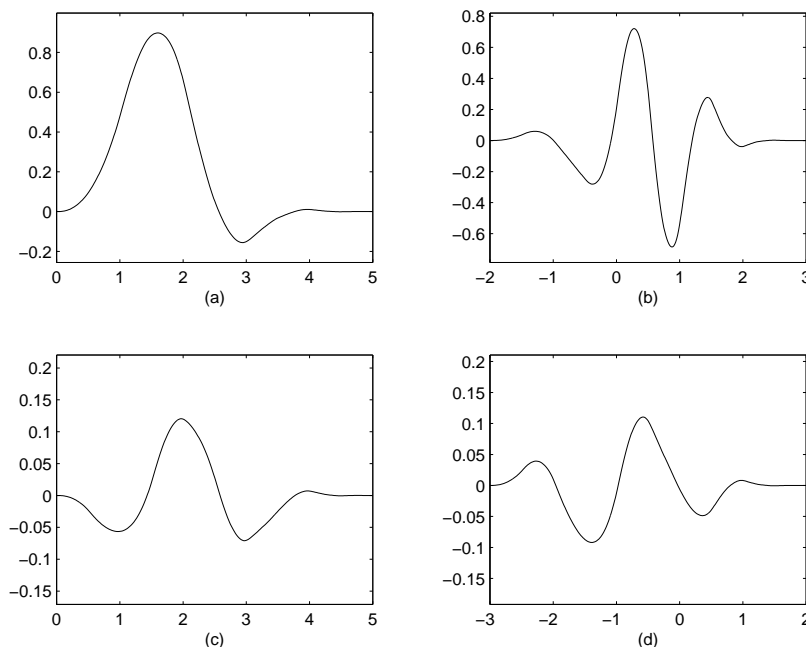
Figure 6. (b), (c) and (d) are the graphs of the mother wavelets of the Type II Pseudo-spline tight framelets derived from the pseudo-spline (4,1) (a).
