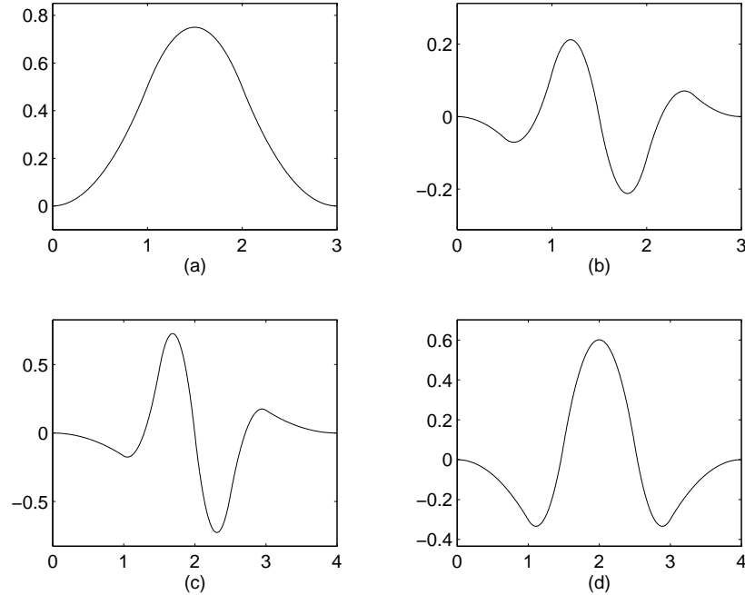
Figure 8. (b), (c) and (d) are the graphs of the symmetric wavelet functions \psi_1 , \psi_2 and \psi_3 corresponding to (A.1) in Example A.1. The tight framelet provides approximation order 3 and has two vanishing moments. The filters are of size (4, 6, 6).
