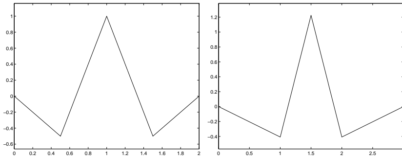
Figure 3. The graphs of the symmetric wavelet functions \psi_1 and \psi_2 derived from the B-spline function of order 2 in Example 2.18. \{\psi_1, \psi_2\} generates a tight framelet, and each of the wavelets has two vanishing moments, and hence the approximation order of the system is \min\{4, 2\} = 2 ; the higher number of vanishing moments than in Example 2.16 leads to sparser wavelet coefficients but does not improve the decay of the error \|Q_n f - f\| for the truncated reconstruction.
