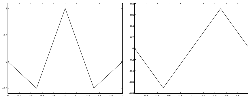
Figure 1. The graphs of the wavelet functions \psi_1 and \psi_2 derived from the B-spline function of order 2 in Example 2.16. \{\psi_1, \psi_2\} generates a tight wavelet frame in L_2(\mathbb{R}) and has vanishing moments of order 1. The framelet system provides approximation order 2, which is optimal for a piecewise-linear system.
