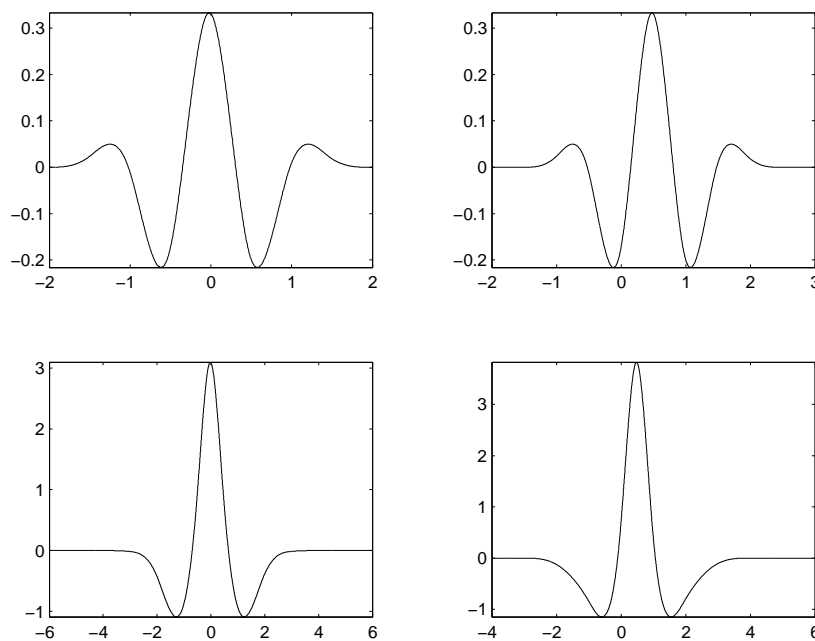
Figure 7. The graphs of the two decomposition wavelets of the example in §6 are depicted in the first row. Both are obtained by applying a 4-order difference to the cubic B-spline. The two reconstruction wavelets are depicted in the second row.
