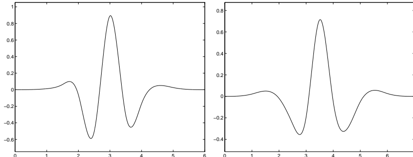
Figure 10. The graphs of the wavelet functions \psi_1 and \psi_2 in Example A.2. \{\psi_1, \psi_2\} generates a wavelet tight frame in L_2(\mathbb{R}) and has vanishing moments of order 4.
