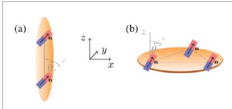
Figure 1: In the quasi-1D setup in (a) the dipolar BEC is confined to the z direction, and in the quasi-2D setup in (b) the dipoles are confined to the x - y plane [2].
