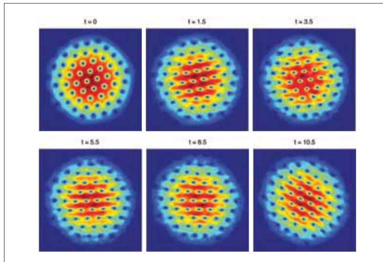
Figure 2: Dynamics of a quantised vortex lattice in a rotating dipolar BEC [5].
